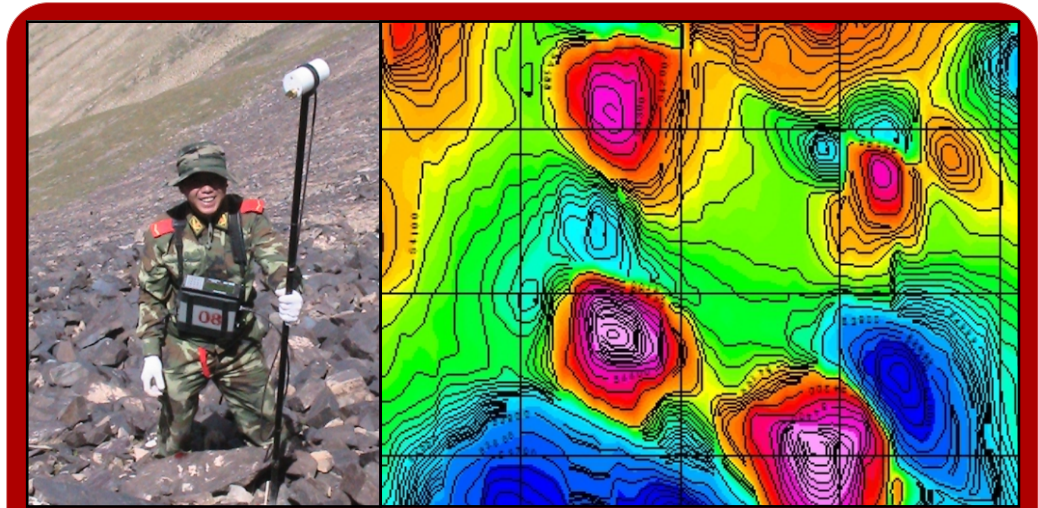
GEM Systems (GSM-19T) Proton Precession system. The image shows a staff-mounted configuration with console, sensor, supporting pole and cables. A backpack-mounted version, and optional GPS are available for hands free operation.
